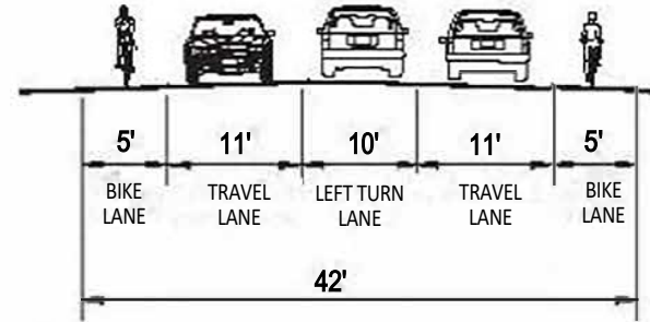
TURNING LANE TYPICAL SECTION JENNINGS TO ENCINAL GLENWOOD TO RINGWOOD
