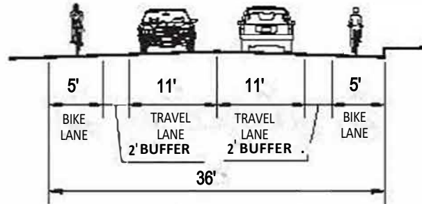
TYPICAL SECTION ENCINAL TO GLENWOOD
