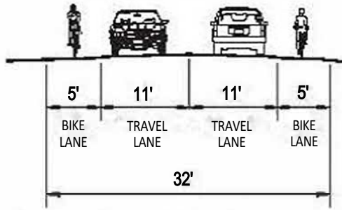
TYPICAL SECTION JENNINGS TO ENCINAL GLENWOOD TO RINGWOOD
